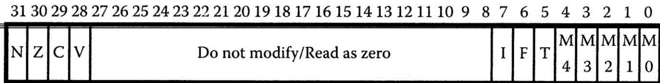
FIGURE 2.4 Format of the program status registers.
